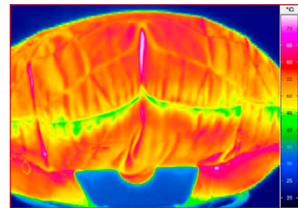
Airbag test
